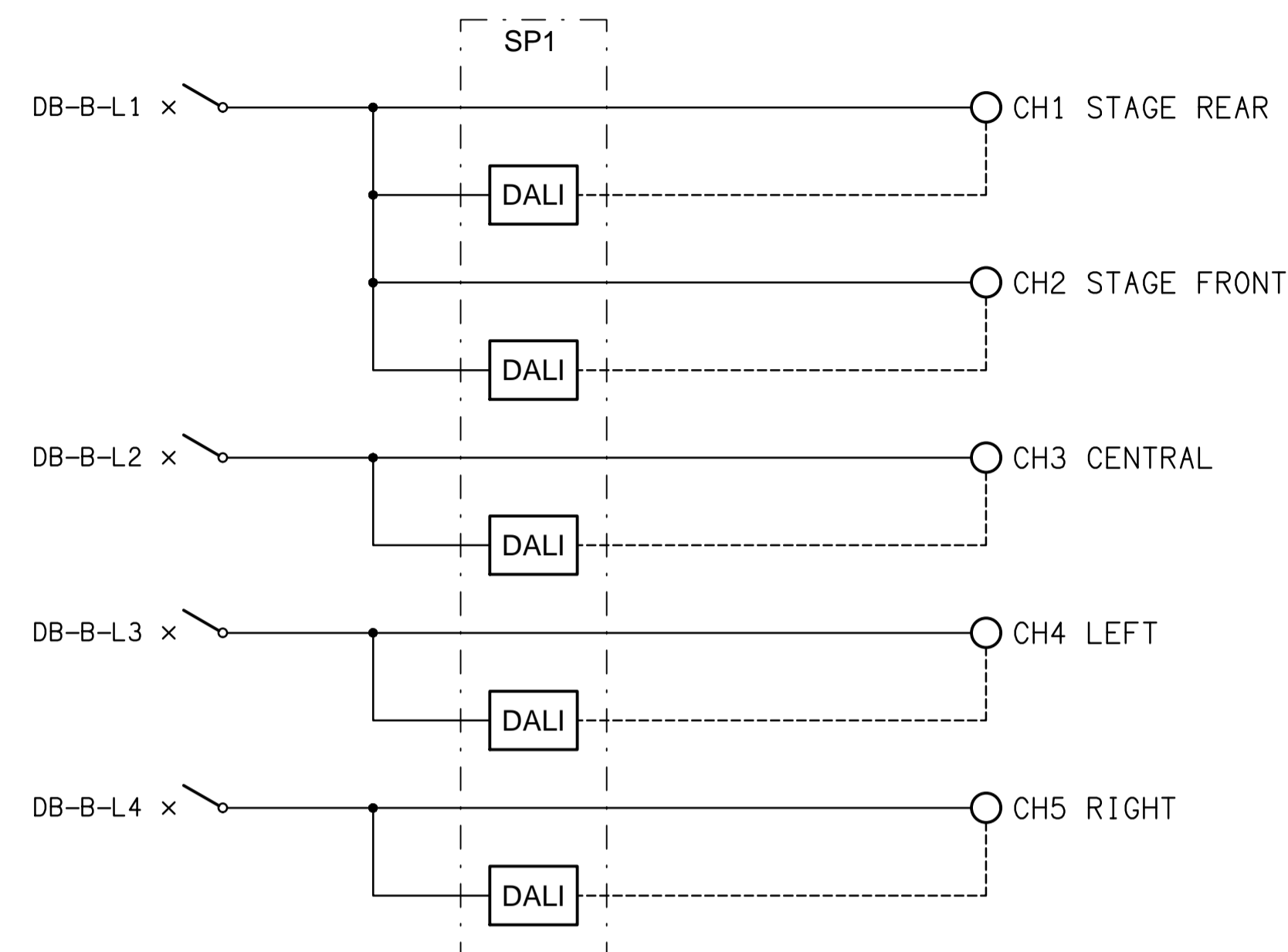
SCHEMATIC SP1 LIGHTING CONTROL NOT TO SCALE
