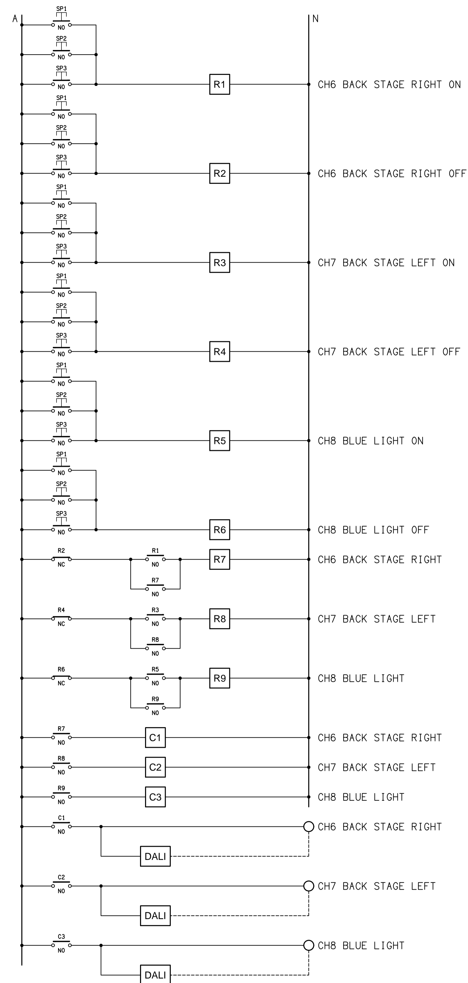
SCHEMATIC LIGHTING CONTROL NOT TO SCALE
